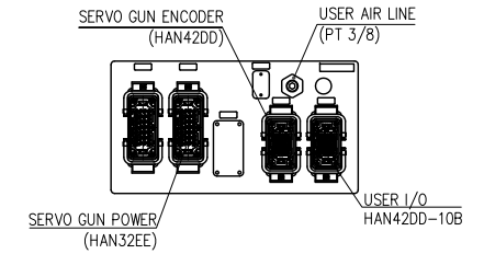
VIEW "C" <For Hi5a Controller> (SCALE : 2/1)
