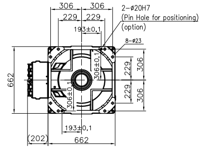
VIEW "B" (SCALE : 1/1)
