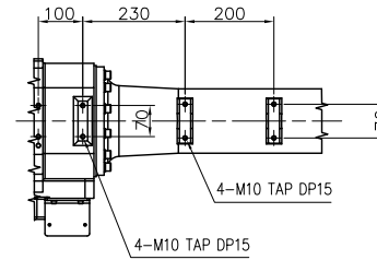
VIEW "E" (SCALE : 2/1)
