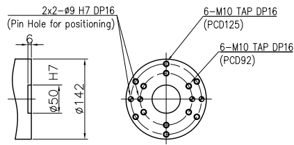
VIEW "A" (SCALE : 4/1)
